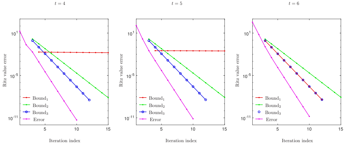
FIGURE 10. Convergence of the BPSD-id (Algorithm 2) in terms of the Ritz value error \theta_t - \lambda_t for t \in \{4, 5, 6\} in Example 5.4 with clustered eigenvalues. The three bounds are based on the multi-step estimates (37), (35) and (36).
