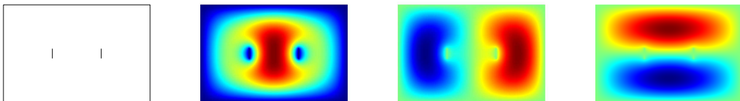
FIGURE 1. Laplacian eigenvalue problem in Example 5.1. The two slits on the domain clearly influence the shapes of eigenfunctions associated with the three smallest operator eigenvalues.
