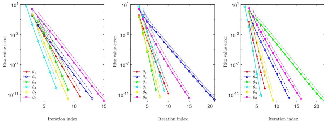
FIGURE 3. Convergence of the BPSD-id (Algorithm 2) in terms of the Ritz value error \theta_t - \lambda_t for computing the six smallest eigenvalues in Example 5.1 with fixed shifts. The error bounds in dotted curves are determined by using Theorem 3.
