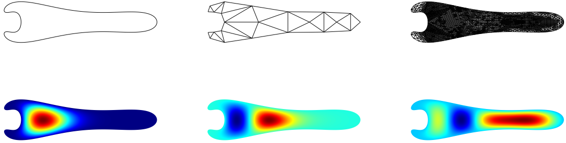
FIGURE 5. Laplacian eigenvalue problem in Example 5.2. The first row displays the domain, the initial grid and an adaptively refined grid. The second row illustrates approximate eigenfunctions associated with the three smallest operator eigenvalues. The corresponding residuals are used for the grid refinement.
