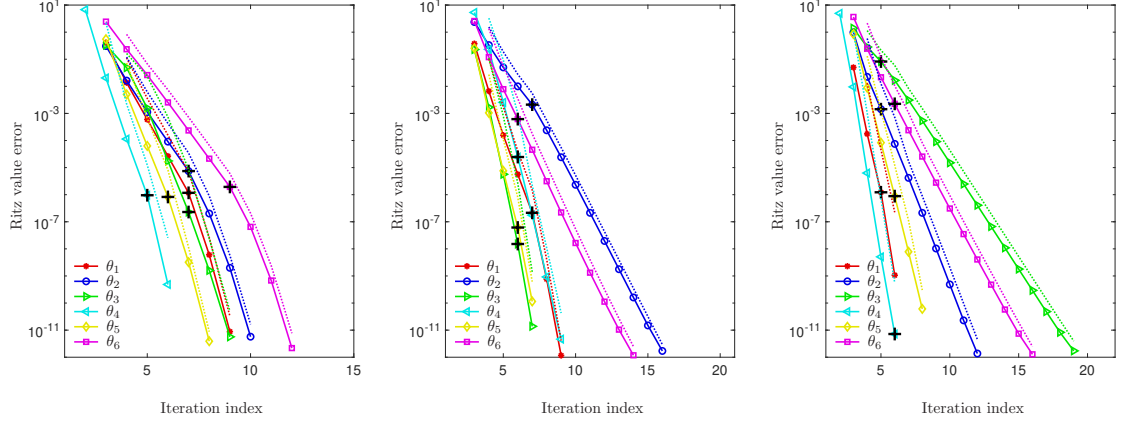
FIGURE 4. Convergence of the BPSD-id (Algorithm 2) in terms of the Ritz value error \theta_t - \lambda_t for computing the six smallest eigenvalues in Example 5.1 with dynamic shifts.
