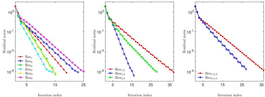
FIGURE 2. Convergence of the BPSD-id (Algorithm 2) in terms of the residual norm \|R(:, 1:k)\|_{S^{-1}} for computing the six smallest eigenvalues in Example 5.1. The pair \{k, \tilde{k}\} is \{1, 2\} (left), \{2, 3\} (center) and \{3, 4\} (right).
