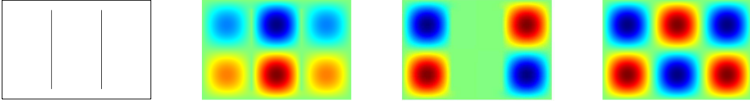
FIGURE 9. Laplacian eigenvalue problem in Example 5.4. The eigenfunctions associated with the fourth to sixth smallest operator eigenvalues are displayed.
