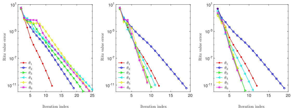
FIGURE 6. Convergence of the BPSD-id (Algorithm 2) in terms of the Ritz value error \theta_t - \lambda_t for computing the six smallest eigenvalues in Example 5.2. Left: Using ichol for generating the preconditioner with a constant shift. Center: Modifying the preconditioner by MINRES with the tolerance 0.1. Right: Modifying the preconditioner by MINRES with the tolerance 0.01.
