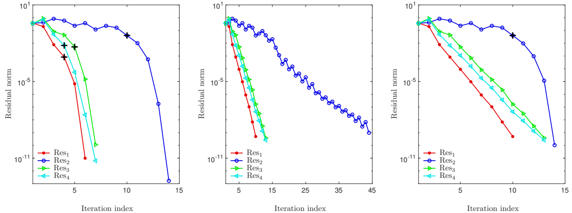
FIGURE 7. Convergence of a weakened form of BPSD-id using only one residual vector and an relative residual norm for computing the four smallest eigenvalues in Example 5.3. The preconditioner is constructed by MINRES with certain shifts. Left: Enabling dynamic shifts. The first dynamic step is marked by “+”. Center: Using fixed shifts only. Right: Enabling dynamic shifts when the convergence in the first steps is slow.
