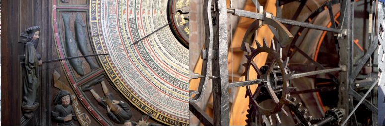
Details of the calendar disk and of the main clockwork. We regret that there is no public access to the inside of the clock.
